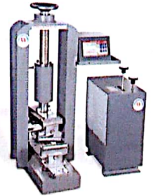
Flexural Testing
