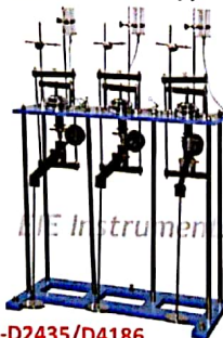
Consolidation Test Apparatus
