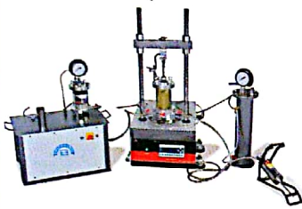
Triaxial Test Apparatus
