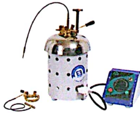
Pensky Marten Flash Point Apparatus
