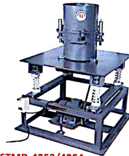
Relative Density Test Apparatus
