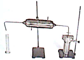
Distillation Apparatus for Emulsified Asphalt
