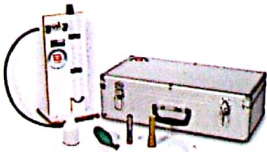
Blaine Air Permeability Apparatus
