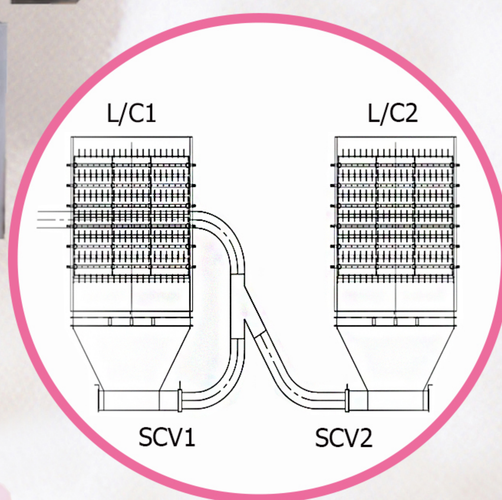
2 Point trash dust evacuation System
