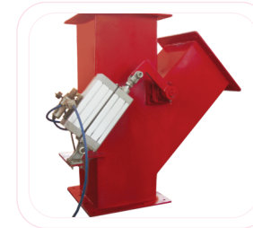
FIRE DIVERTER
