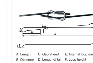
A: Length C: Gap at end E: Internal loop size B: Diameter D: Length of tail F: Loop height
