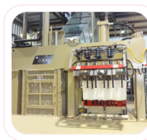
BAJAJ CONTINENTAL 9300 BALE PRESS Capacity - 45, 60 & 90 Bales Per Hour
